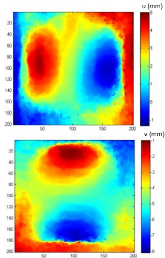
Defect detection on composites with DIC
