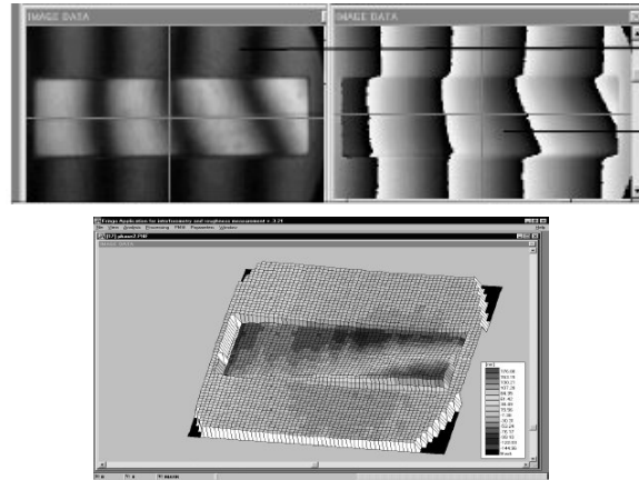
Shape measurement with laser interferometry
