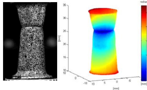
360° DIC measurement during tensile testing
